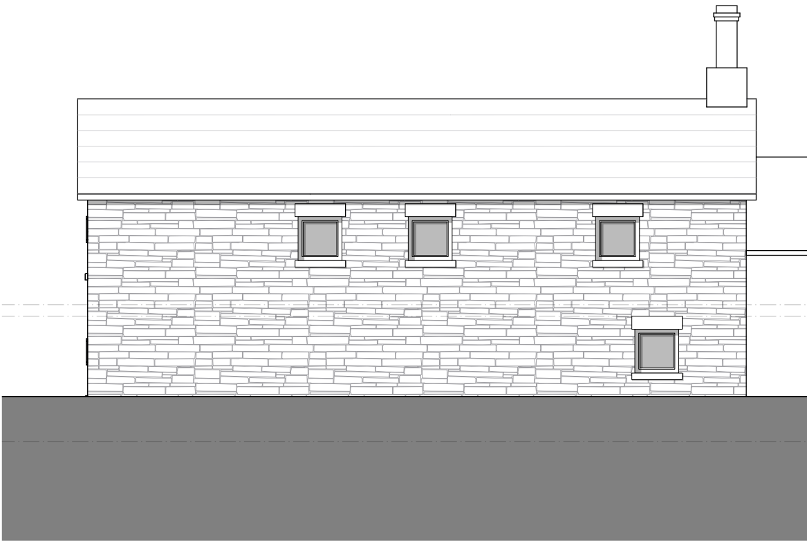
proposed north (front) elevation
