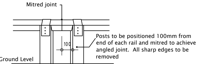
ANGLED JOINT
