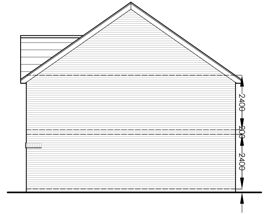
Gable Elevation
