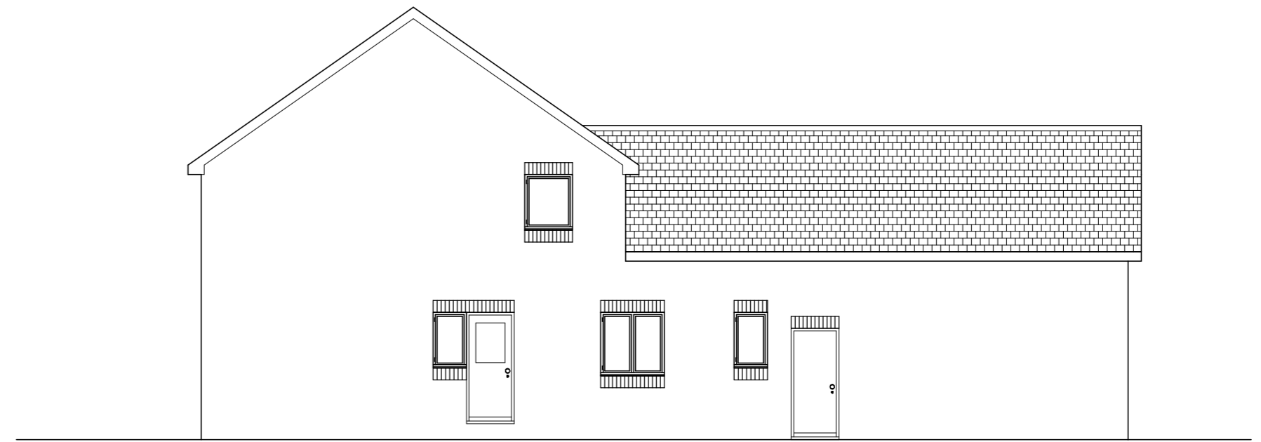
REAR ELEVATION
