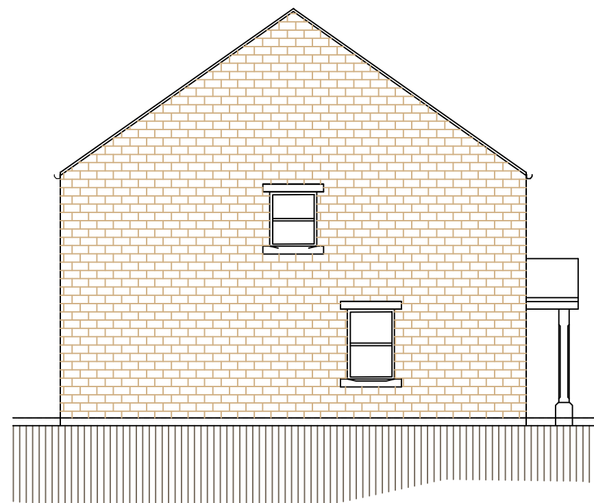
WEST ELEVATION
