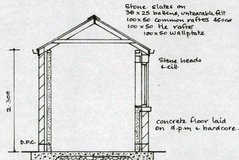
SECTION
