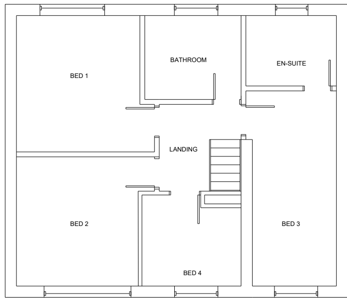
FIRST FLOOR - EXISTING
