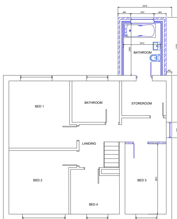
FIRST FLOOR - PROPOSED
