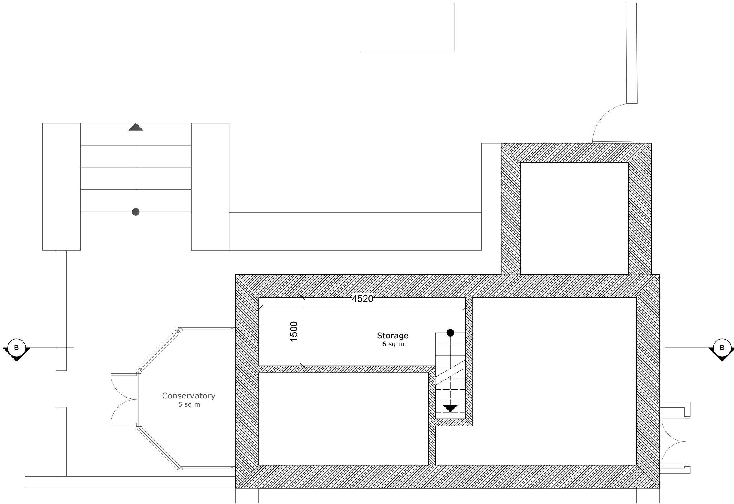
1 Existing Lower Ground Floor Plan Scale: 1:50
