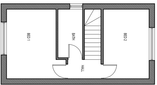
EXISTING FIRST FLOOR PLAN SCALE 1:100
