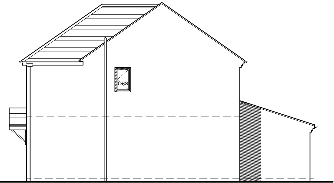
SIDE ELEVATION
