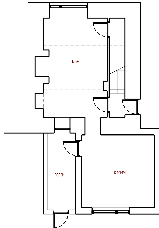
Ground Floor Plan - Existing
