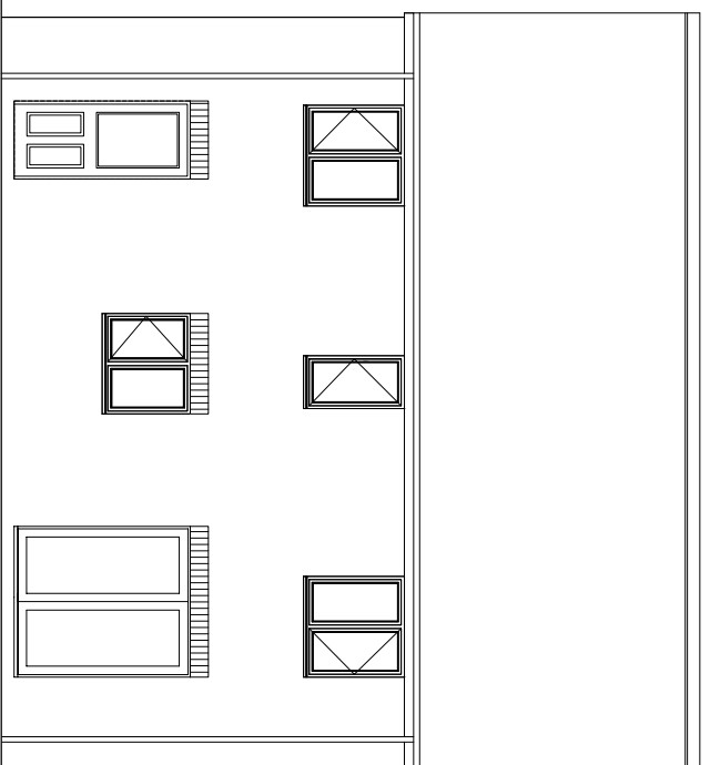
Rear Elevation
