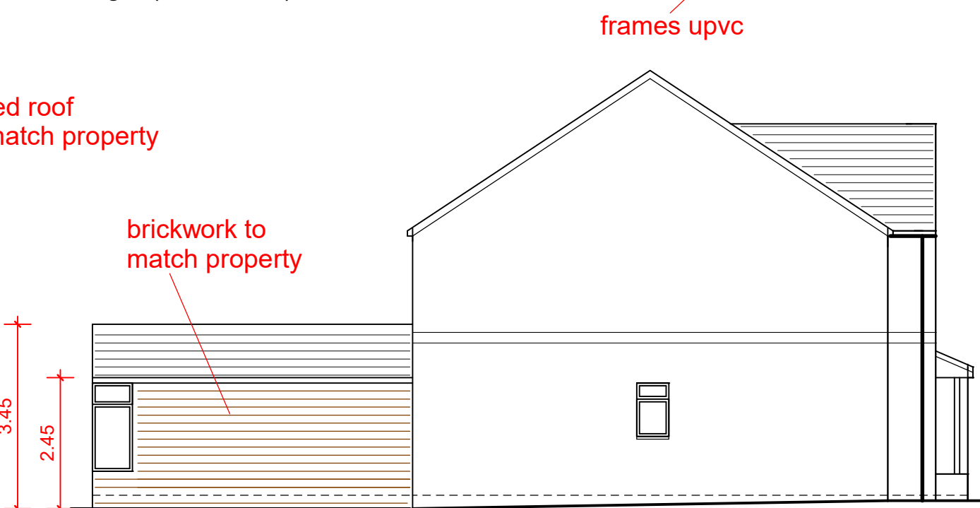
left (north east) elevation
