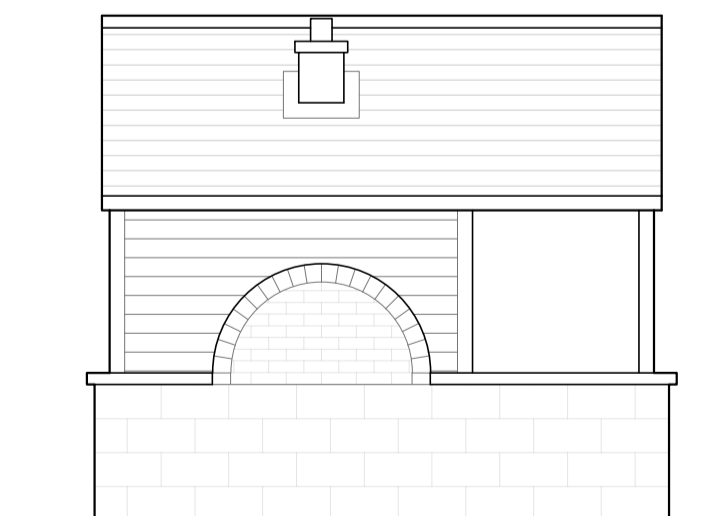
PROPOSED HUT SIDE ELEVATION (NORTH) Scale - 1: 50 @ A1
