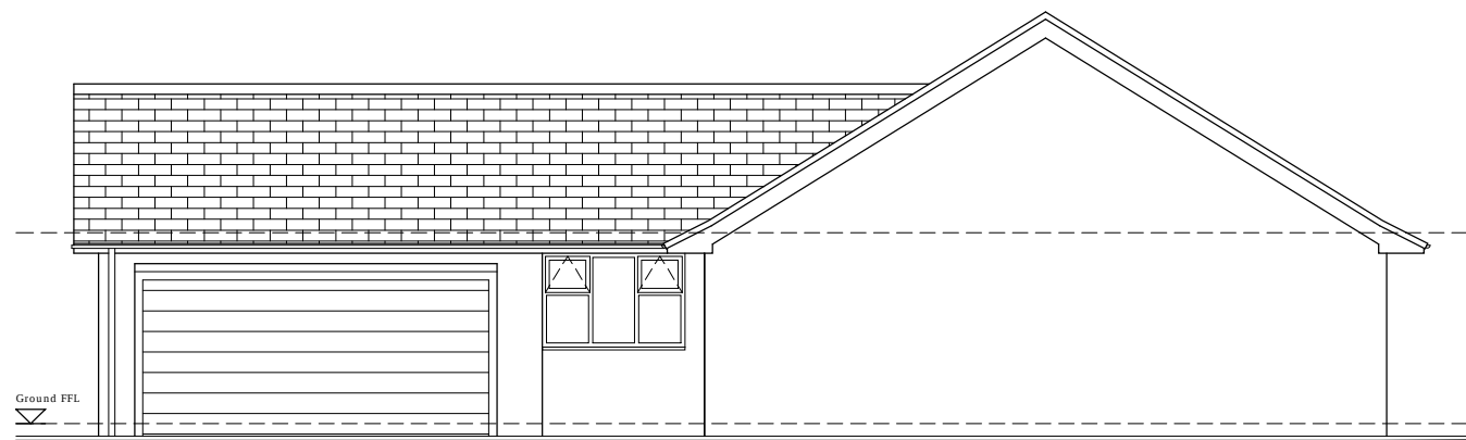
EXISTING RH SIDE ELEVATION 1:100
