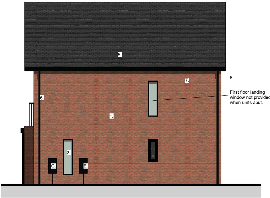
Typical Right elevation
