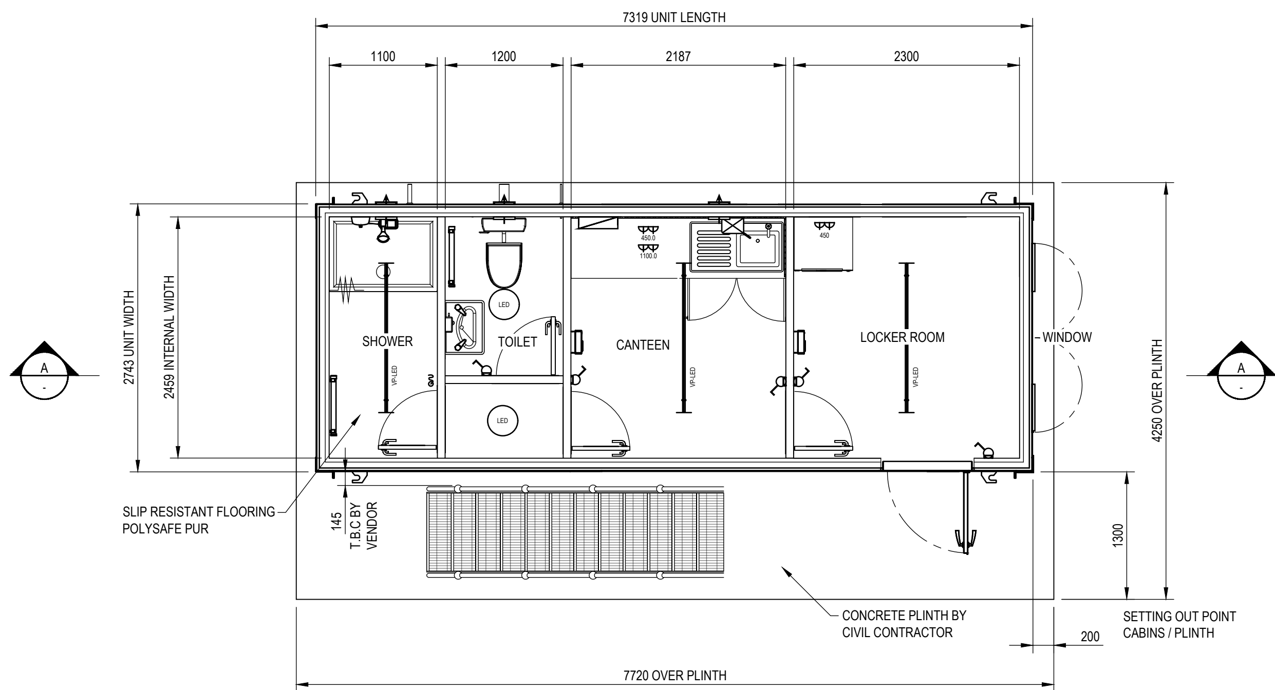
FLOOR PLAN ON LEVEL 0
