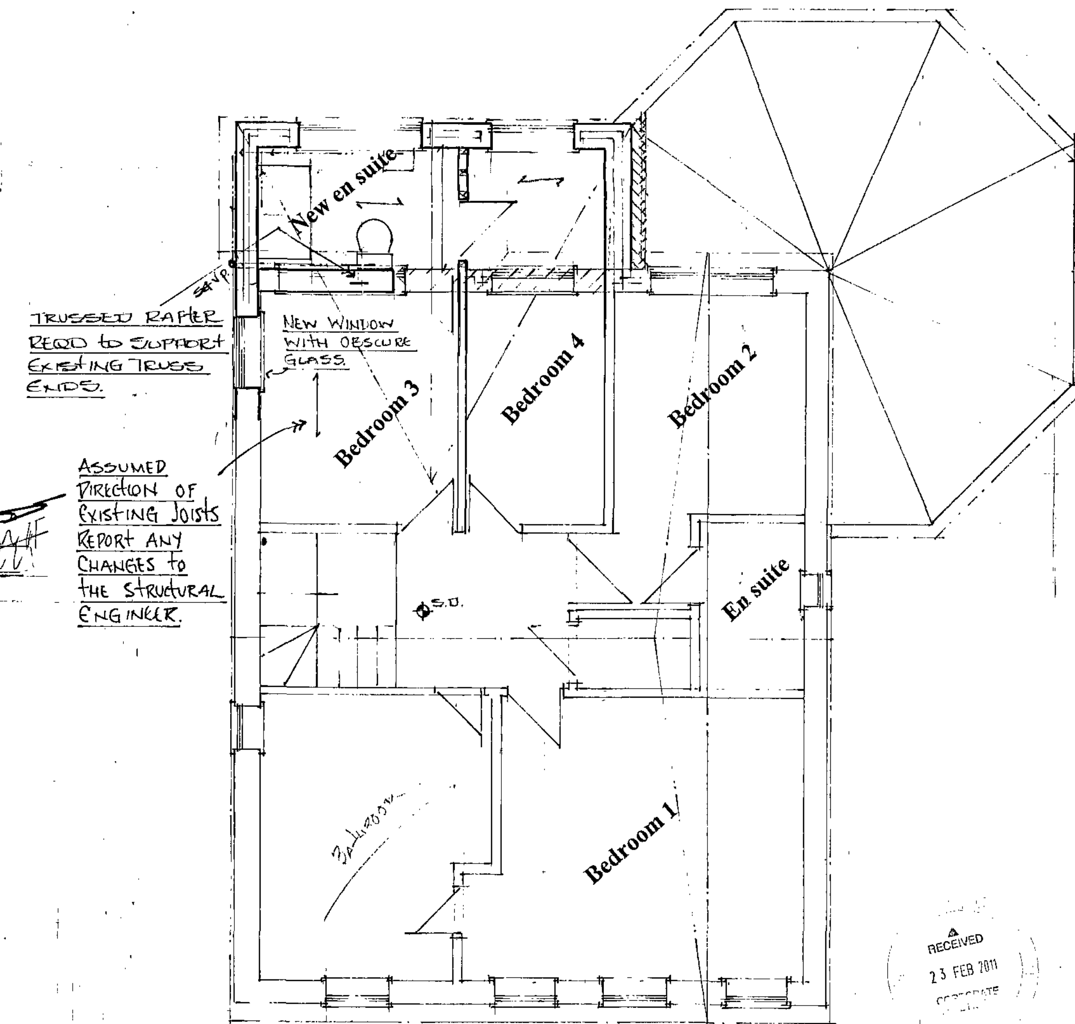
Existing / Proposed First Floor Layout
