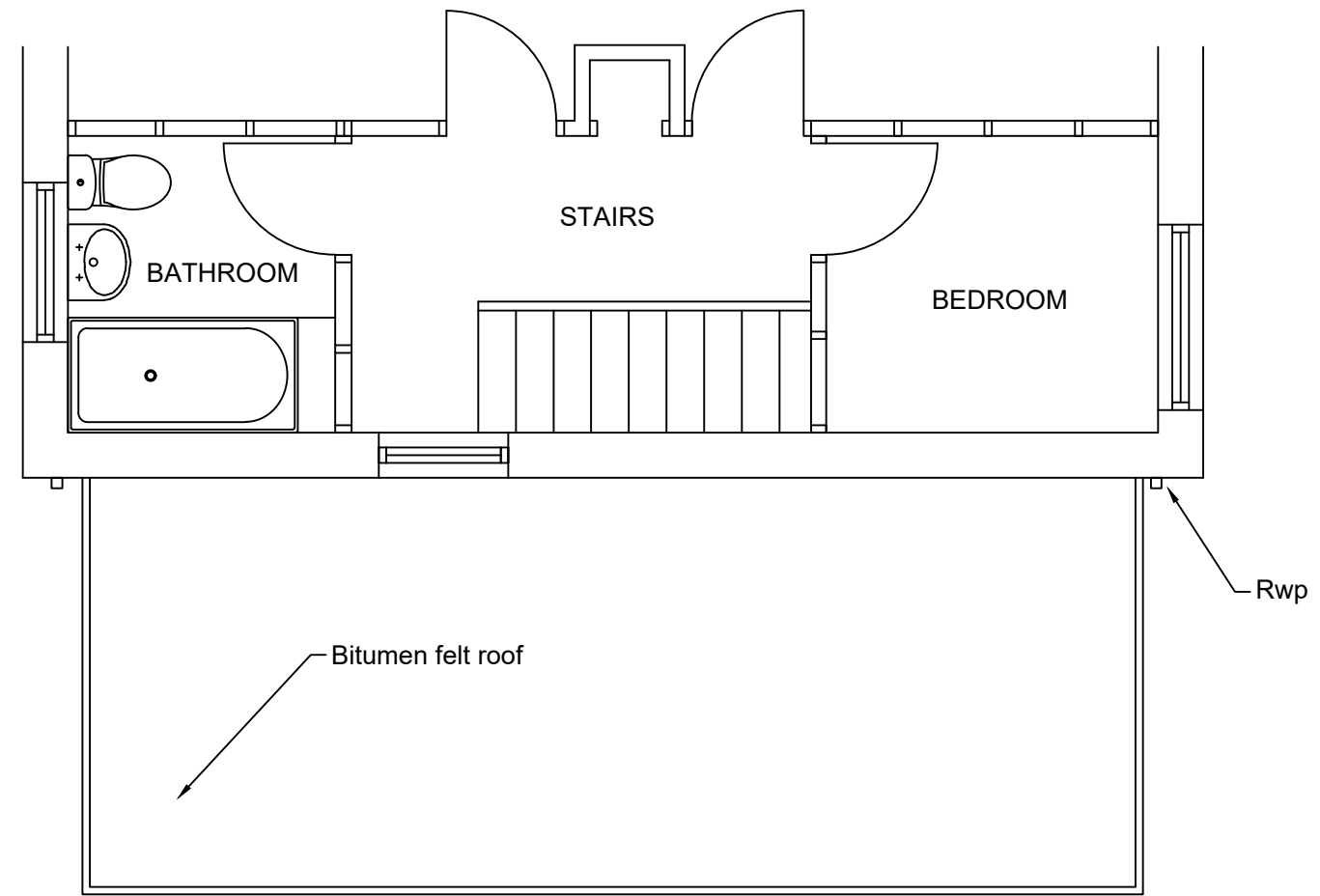
EXISTING FIRST FLOOR PLAN 1:50
