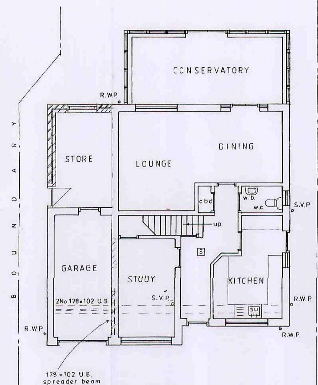
PROPOSED G.F. PLAN
