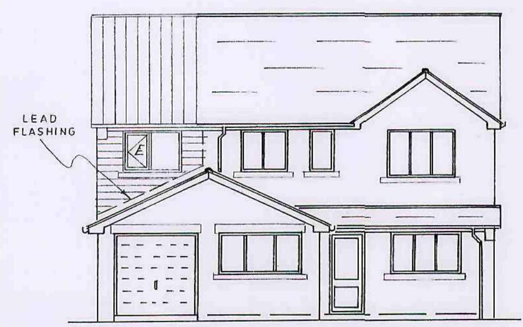
PROPOSED FRONT
