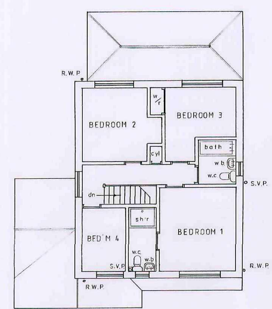
EXISTING F.F. PLAN
