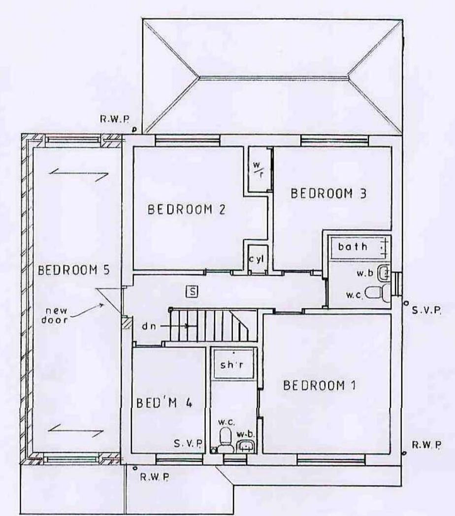
PROPOSED F.F. PLAN
