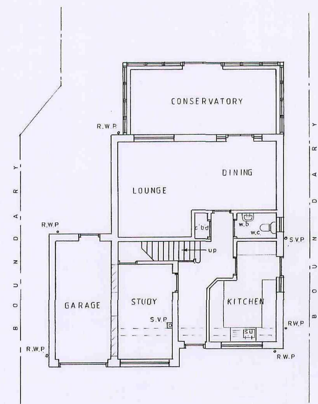
EXISTING G.F. PLAN
