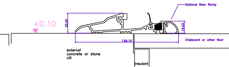
TYPICAL THRESHOLD DETAIL (Using Stormguard Proline AM3 Cill)
