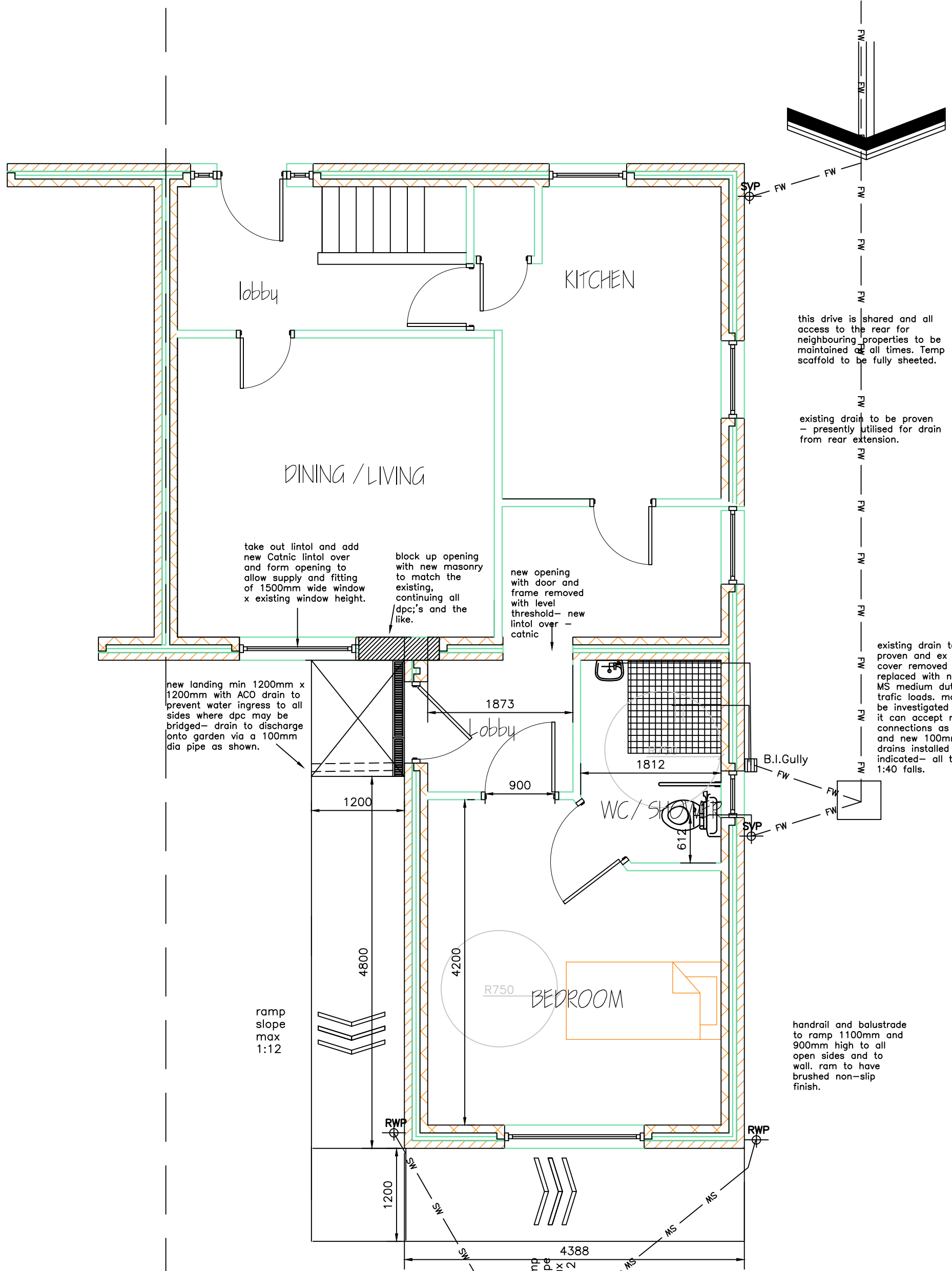
PROPOSED GF PLAN
