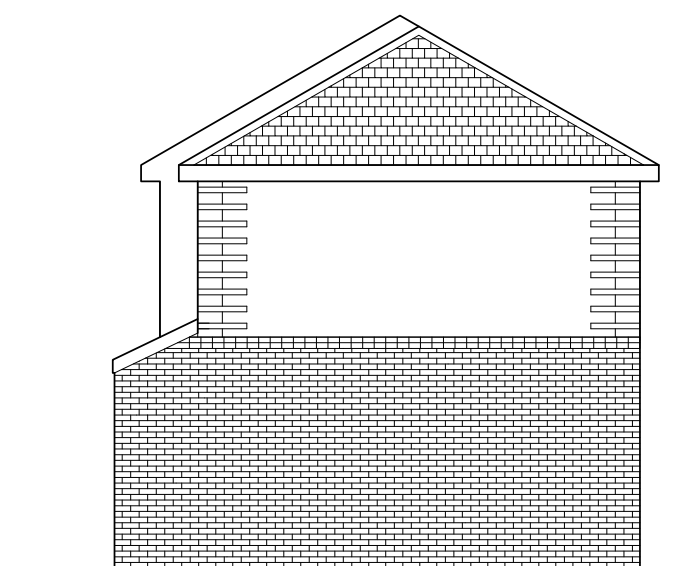
SIDE ELEVATION
