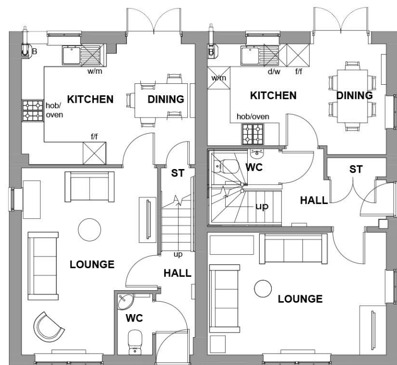
GROUND FLOOR PLAN MAIDSTONE MORESBY
