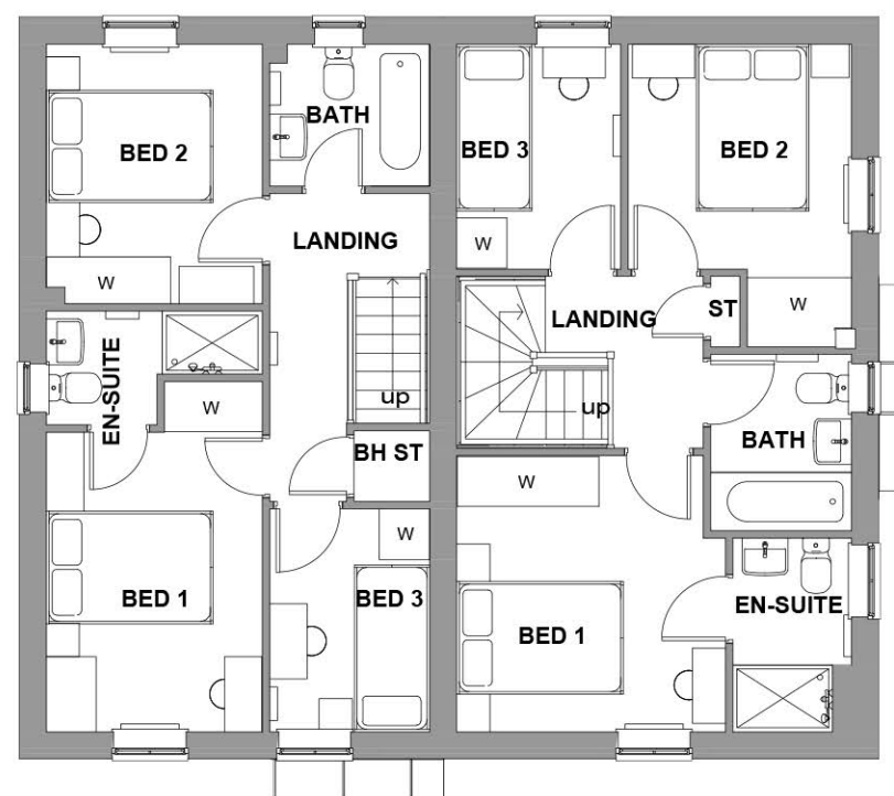
FIRST FLOOR PLAN MAIDSTONE MORESBY
