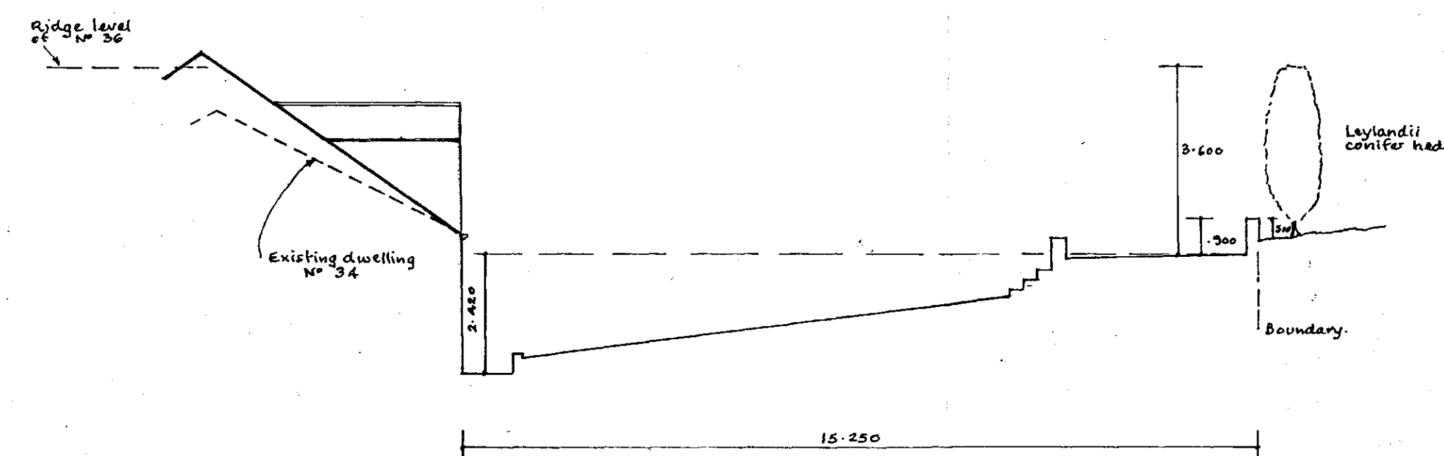
CROSS SECTION 1-100
