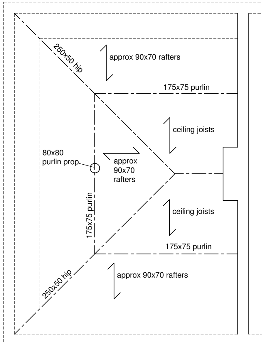
EXISTING ROOF STRUCTURE PLAN
