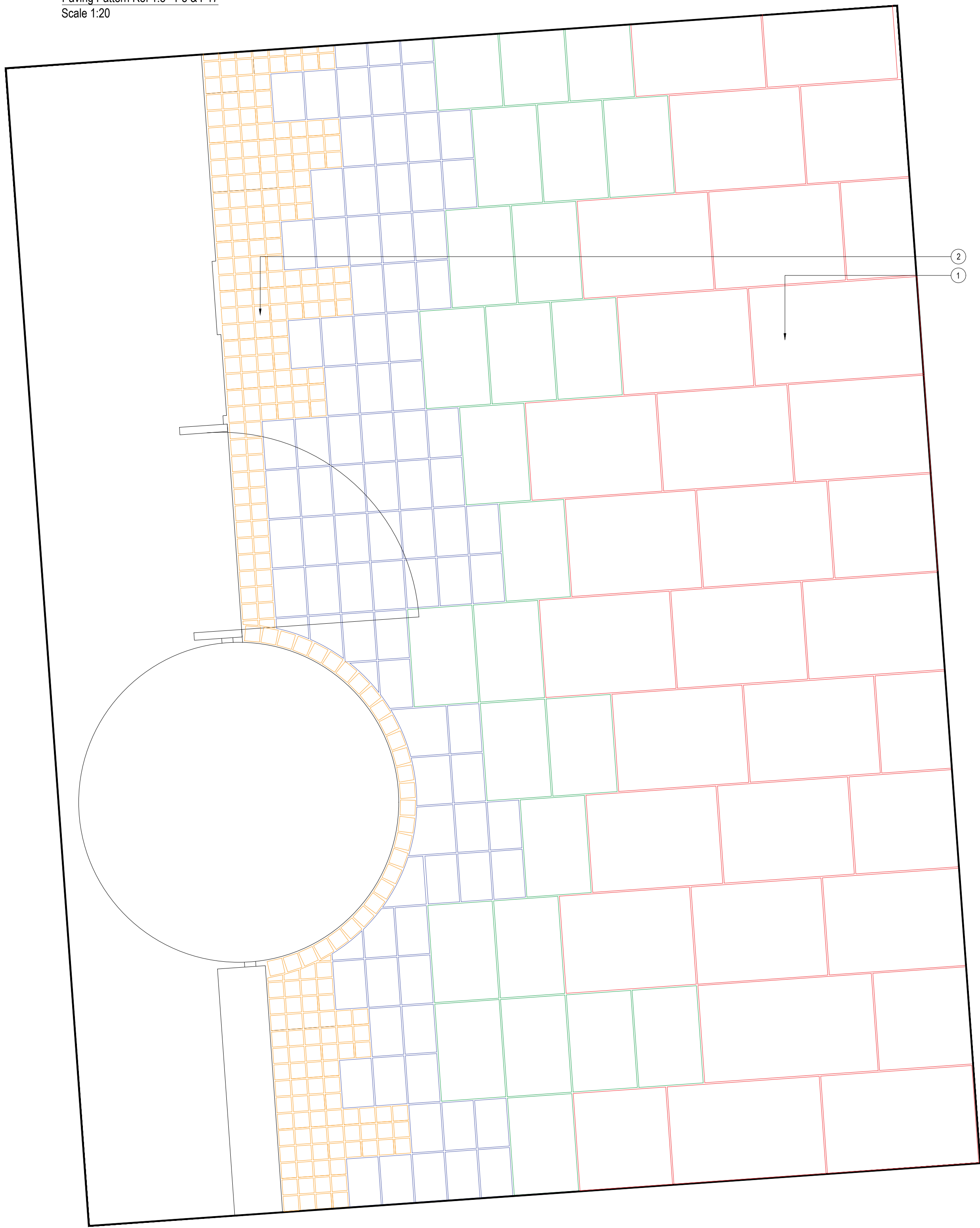
Paving Pattern Ref 1.8 - P5 & P17 Scale 1:20
