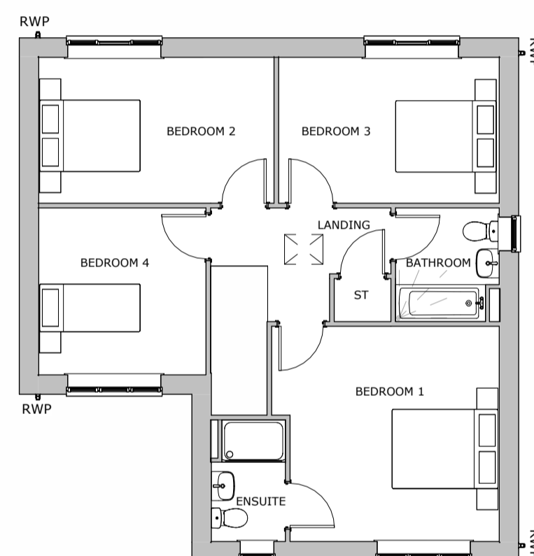
First Floor 1 : 100
