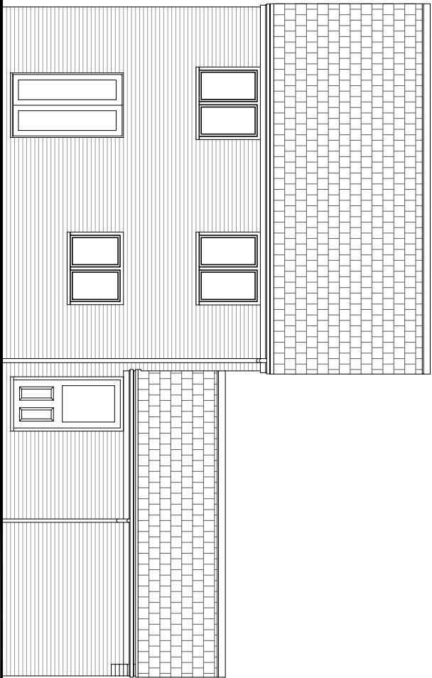
Rear Elevation
