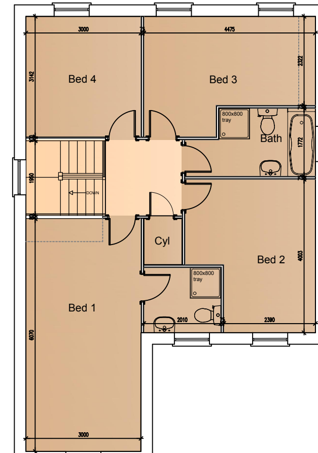
FF Plan
