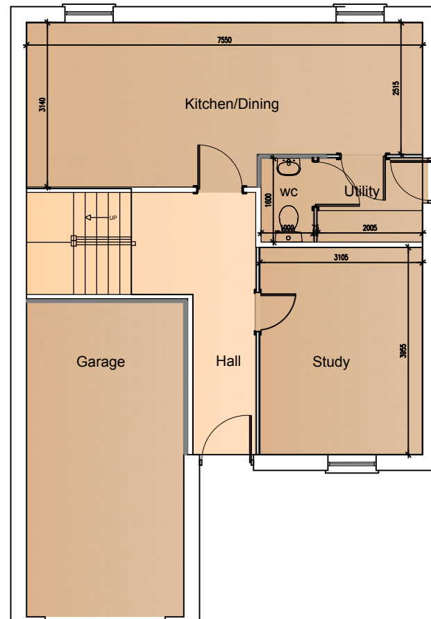
GF Plan
