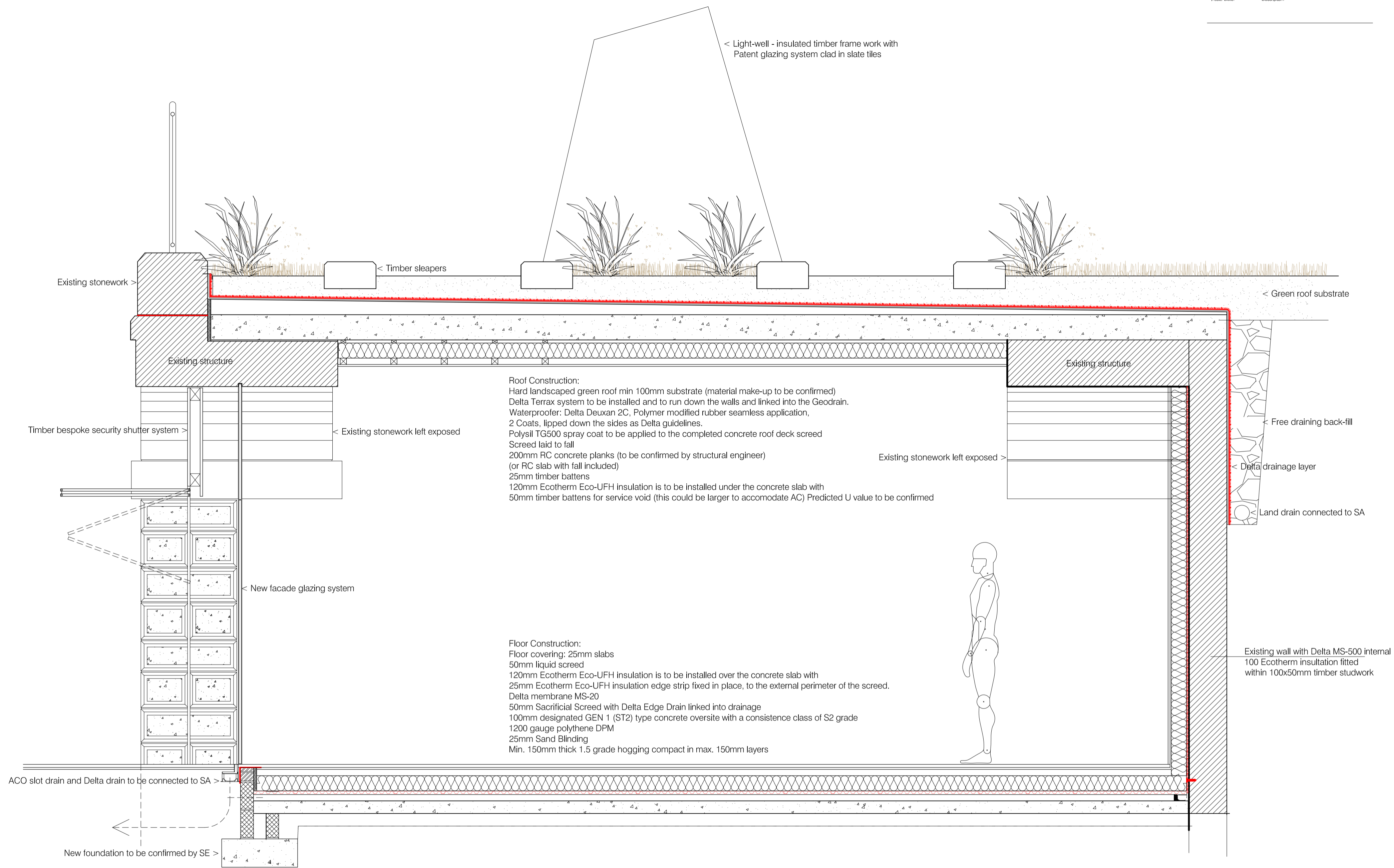
Section AA Through Retail Unit (with shutter in upright position)
