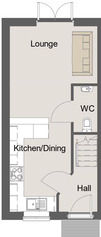
Ground Floor. 1 : 100
