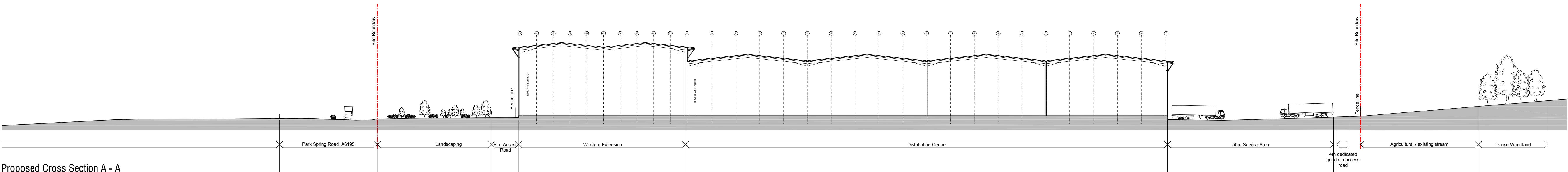
Proposed Cross Section A - A
