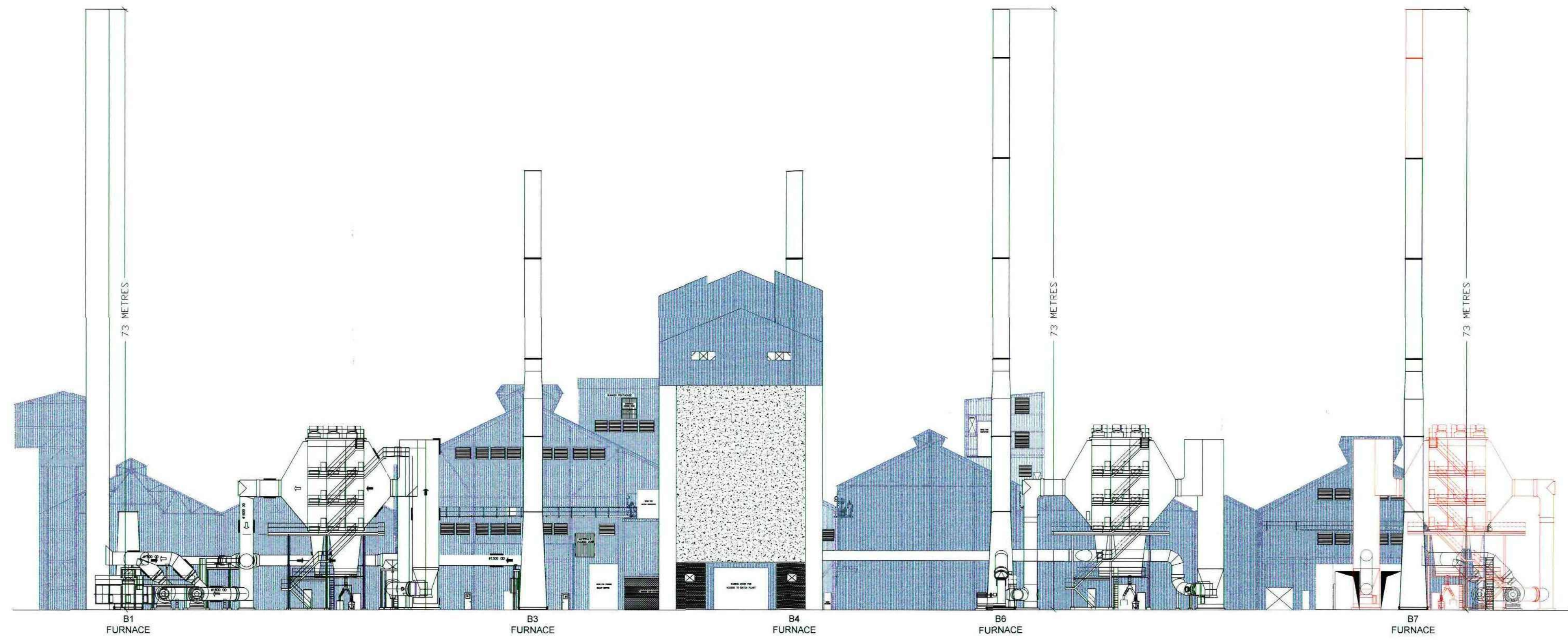
VIEW ON FURNACE GABLE ENDS
