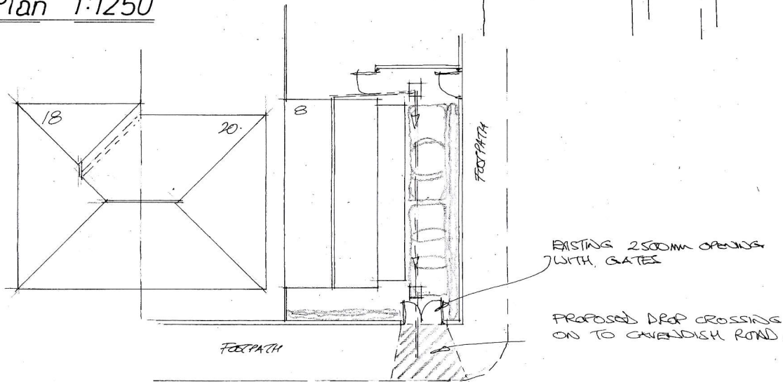
Proposed Drop Crossing Location 1:200
