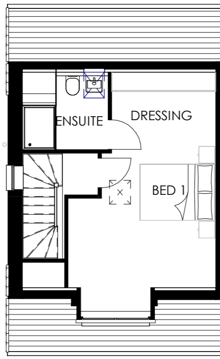
SECOND FLOOR 1 : 100
