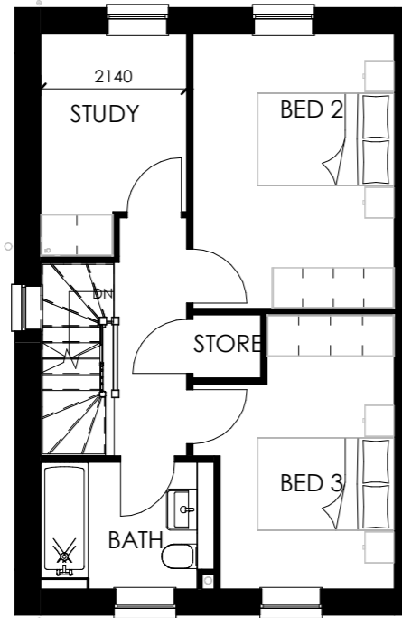
FIRST FLOOR 1 : 100
