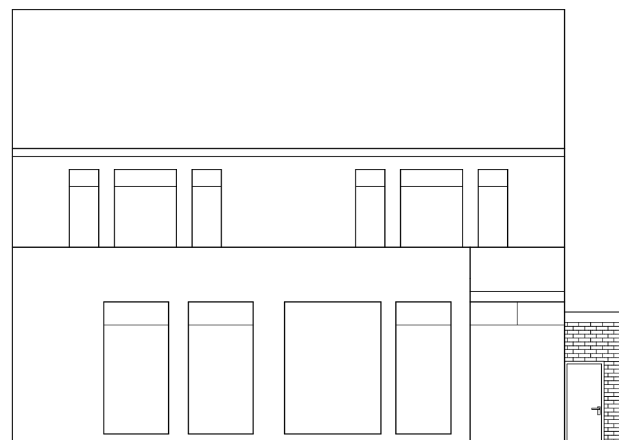
FRONT ELEVATION
