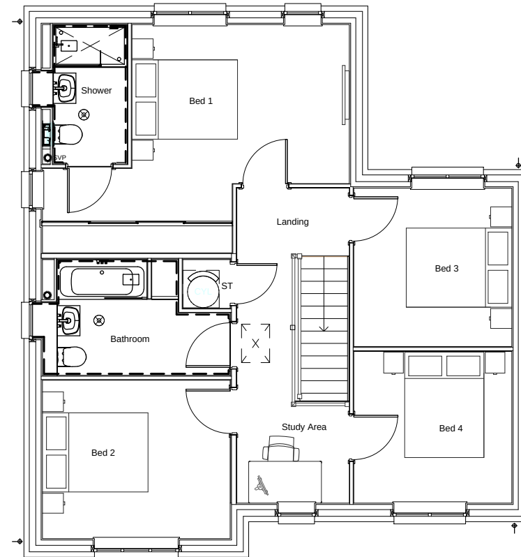
FIRST FLOOR PLAN Norbury
