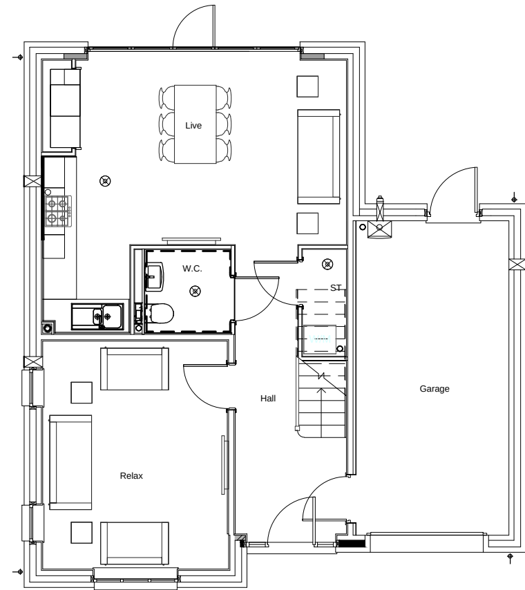
GROUND FLOOR PLAN Norbury
