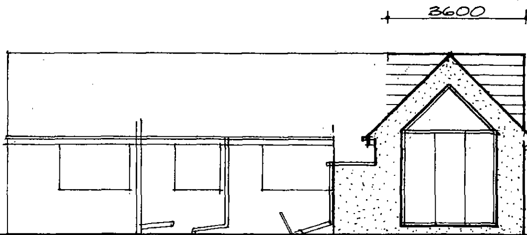
REAR 1:100
