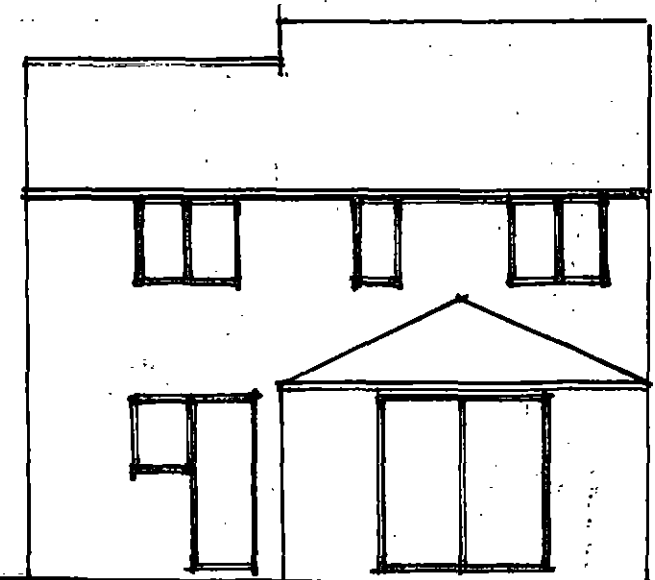
REAR ELEVATION
