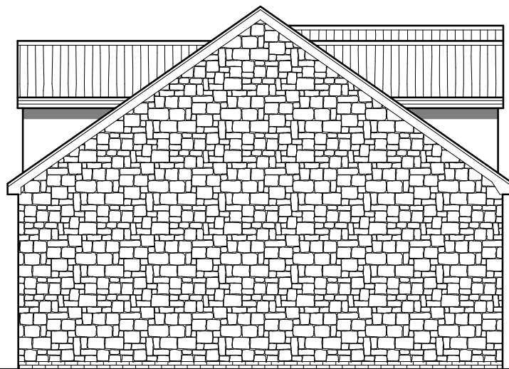
Side Elevation as Proposed.
