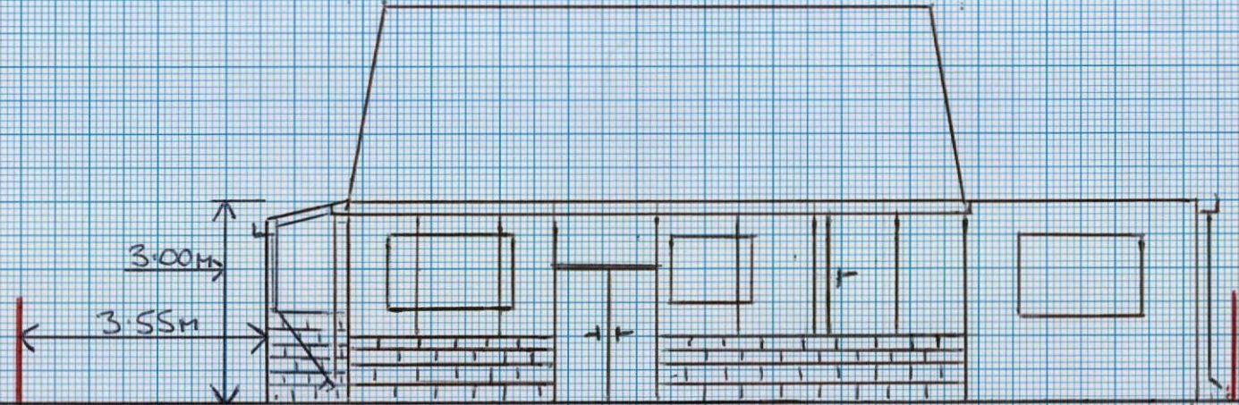
SOUTH ELEVATION PROPOSED PORCH EXTENSION
