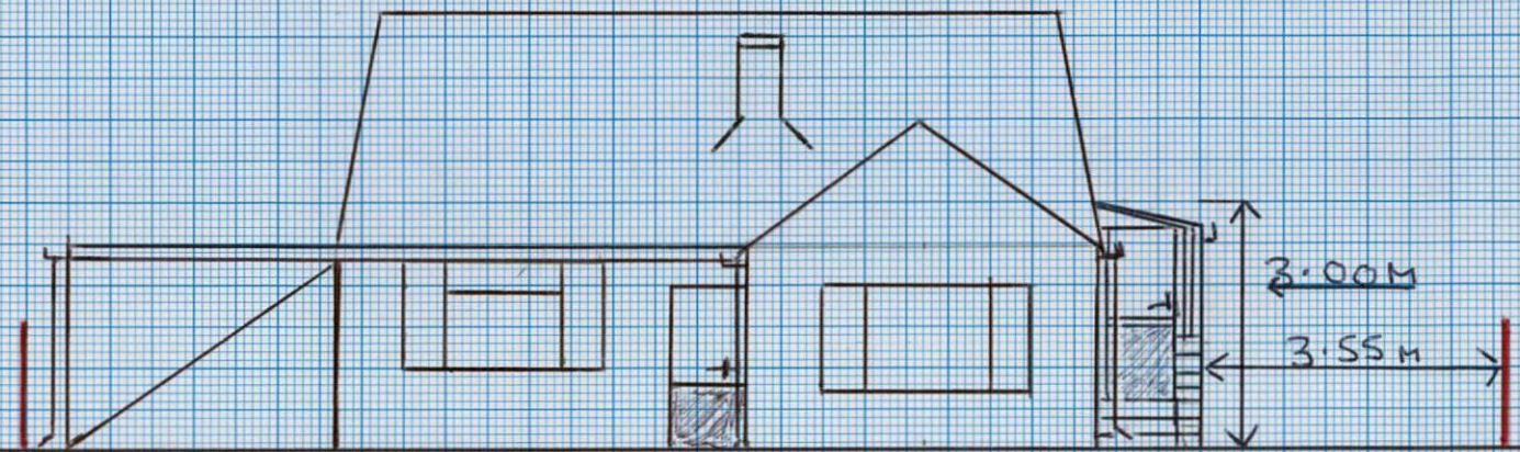
EAST ELEVATION PROPOSED PORCH EXTENSION
