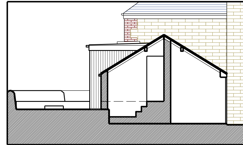
East Elevation/ Section - Proposed
