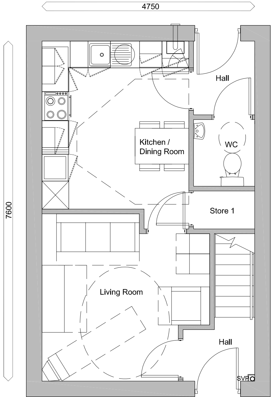
Ground Floor Floor Area: 72m²
