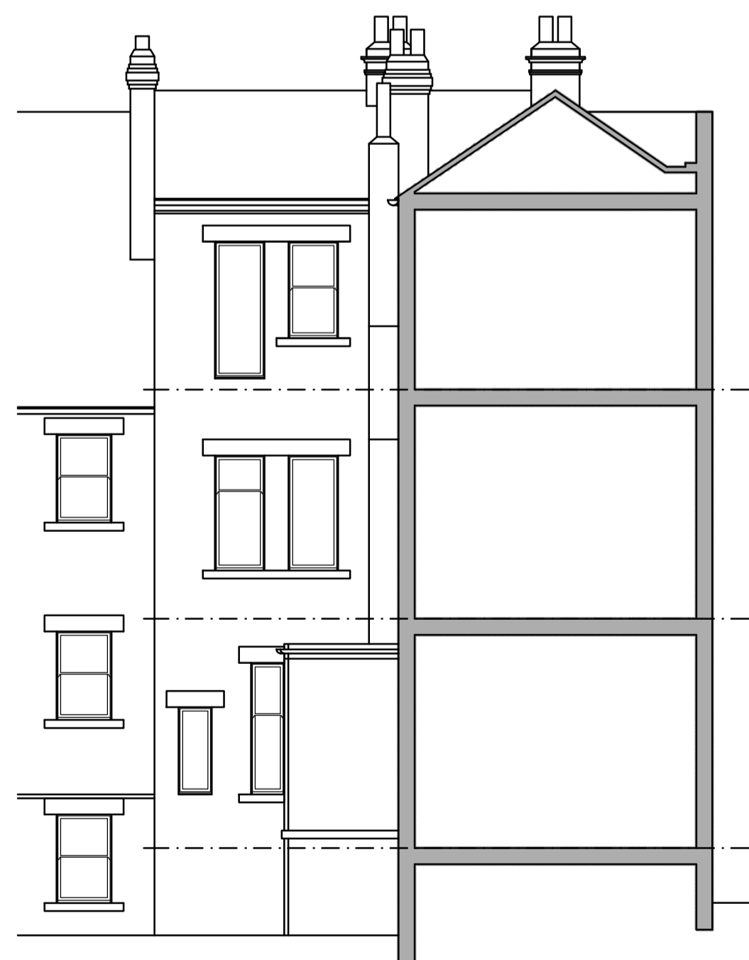
SOUTH ELEVATION - COURTYARD
