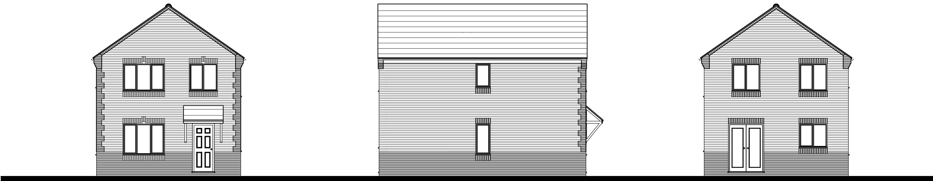
FRONT ELEVATION
