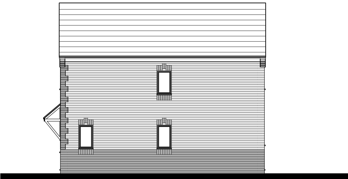
SIDE ELEVATION
