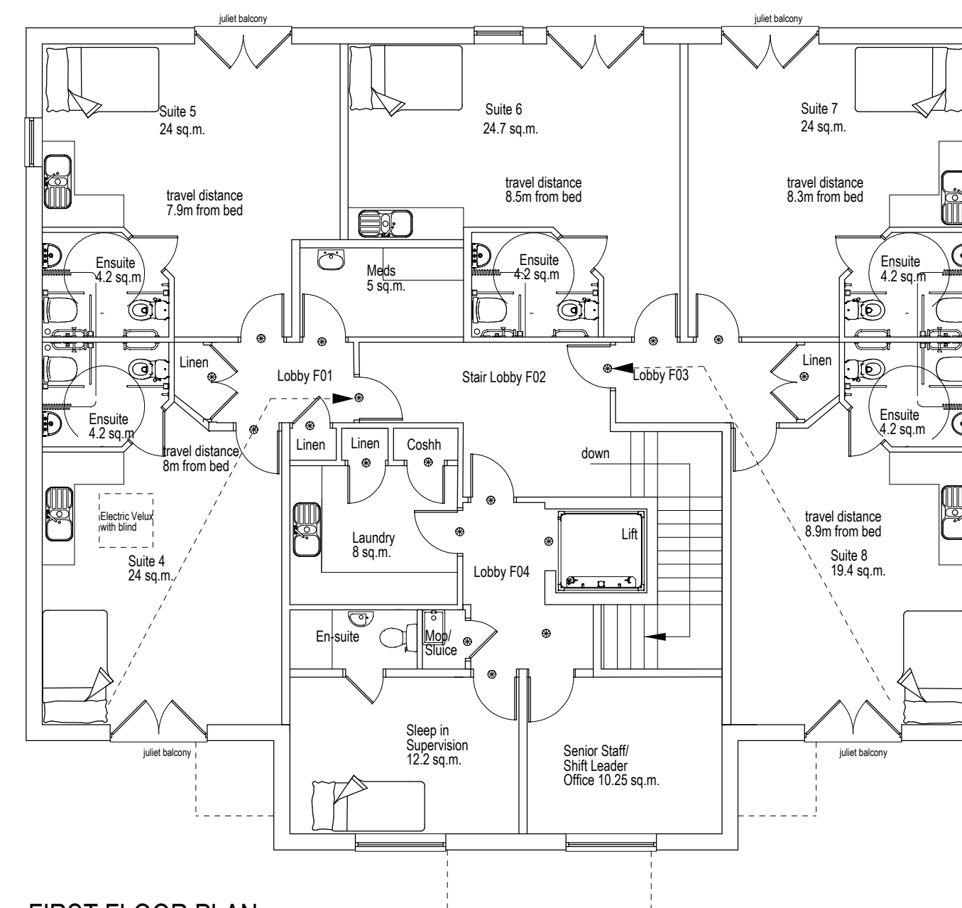
FIRST FLOOR PLAN Phase 1 Core Transitional Rehabilitation Facility First Floor: 235 sq.m
