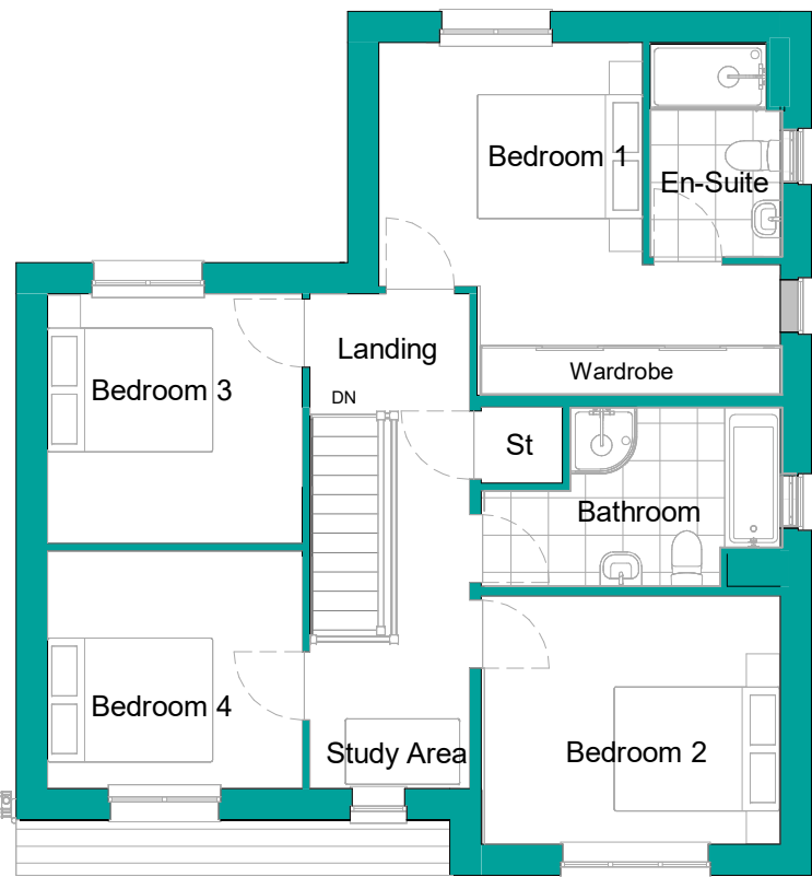
First Floor. 1 : 100
