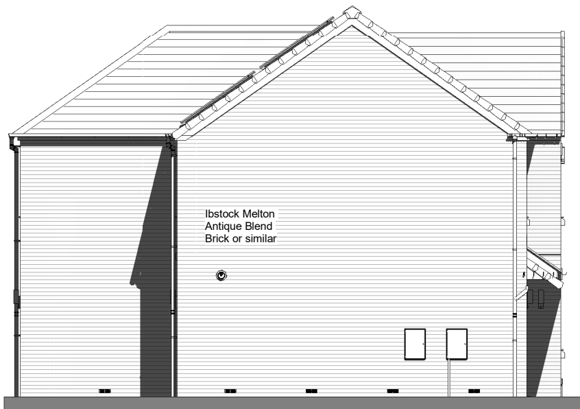
Side Elevation 1 : 100
