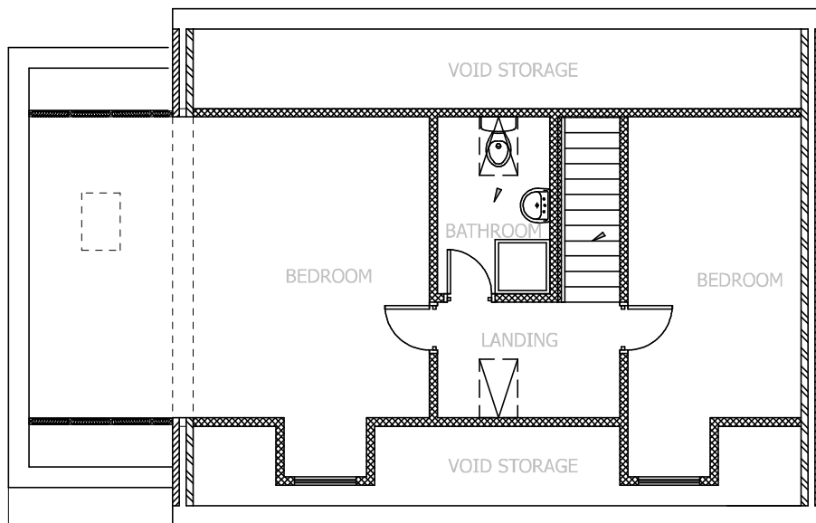
PROPOSED FIRST FLOOR PLAN SCALE 1:100 AT A3
