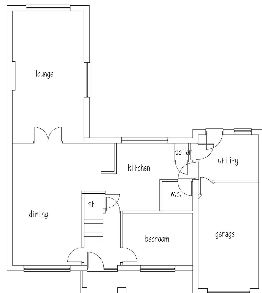
GROUND FLOOR
