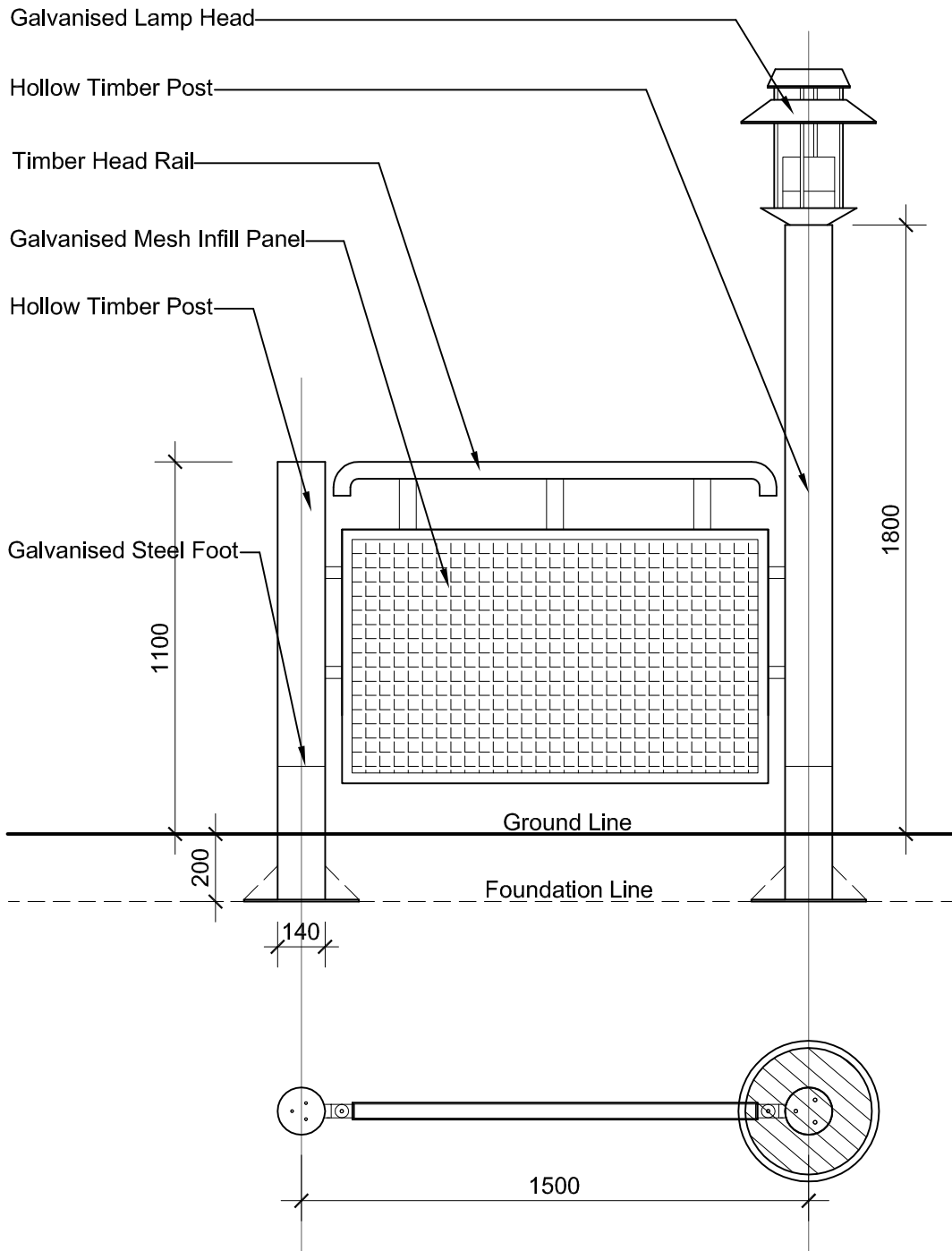
TYPICAL BARRIER & LAMP POST DETAIL - NTS
